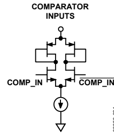
Figure 21. Comparator Inputs
